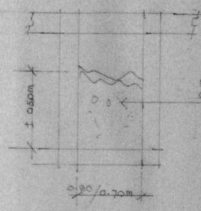
DECLOGGING EXTB. 0.70M RCBC AT N. 1302 ST. / URBANG VELASQUEZ AVE.
