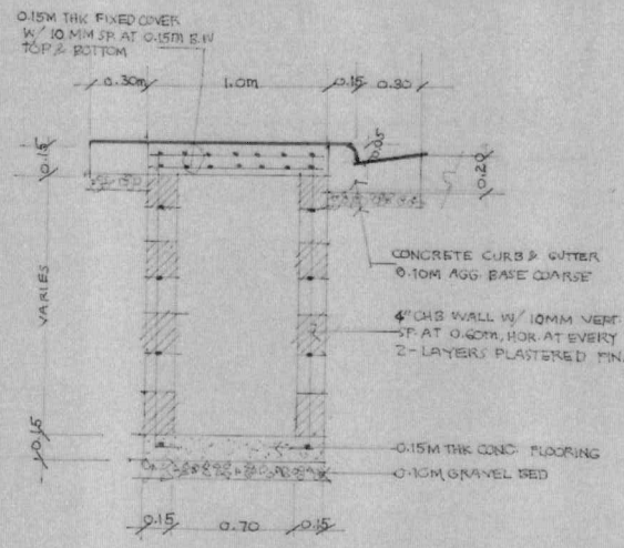
SECTION AT DRIVEWAYS
