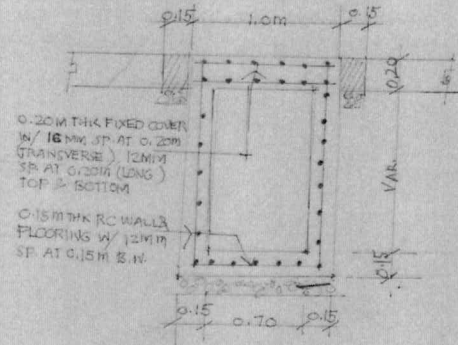
CROSS RCBC CANAL
