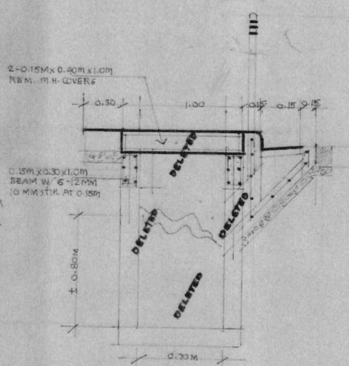
SECTION AT MANHOLE
